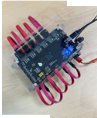
JMS591 multi-bay hardware RAID solution
